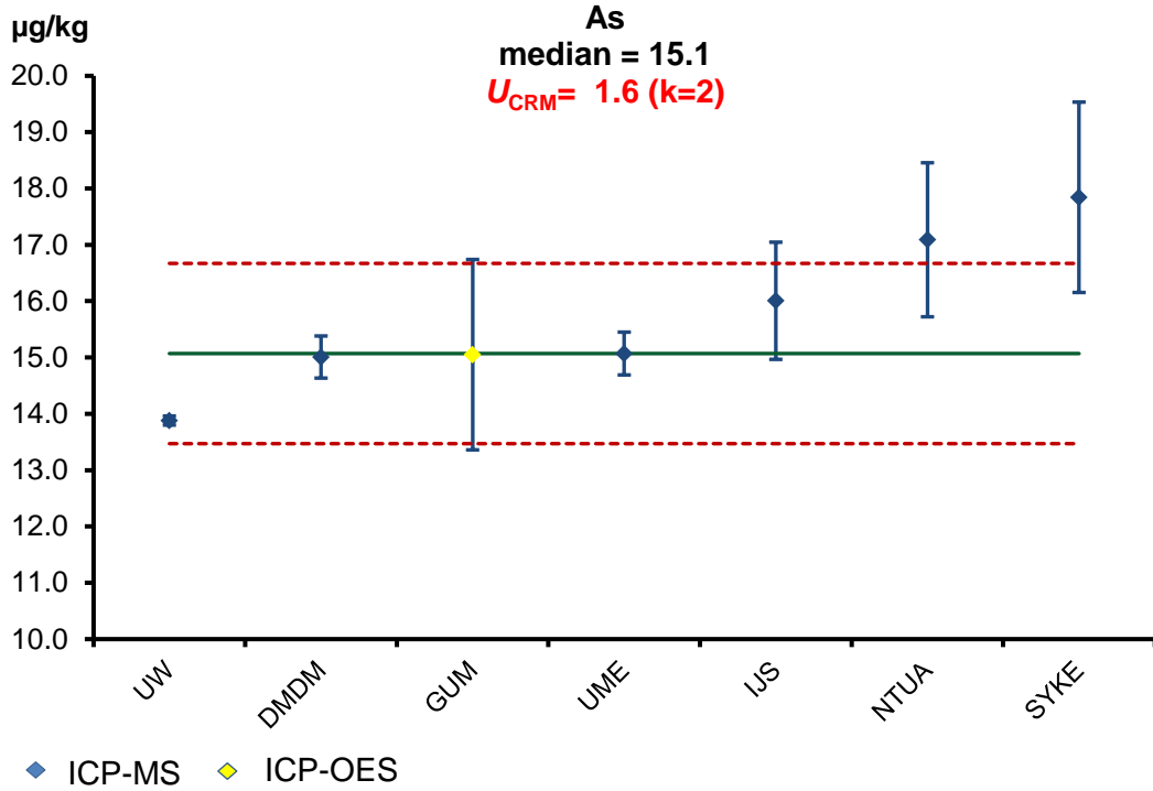
Figure A6.1. Characterization Study Plot for As
