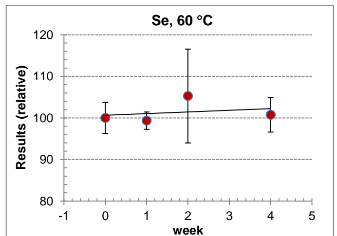
Figure A3.18. STS plot for Se at 60 °C by UME
