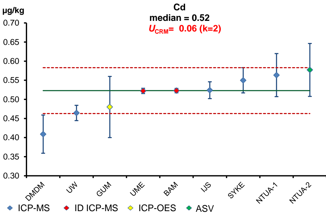
Figure A6.2. Characterization Study Plot for Cd
