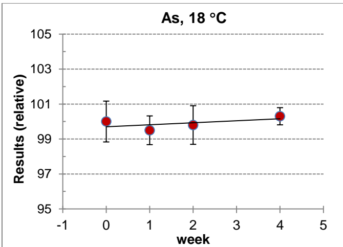
Figure A3.2. STS plot for As at 18 °C by IJS
