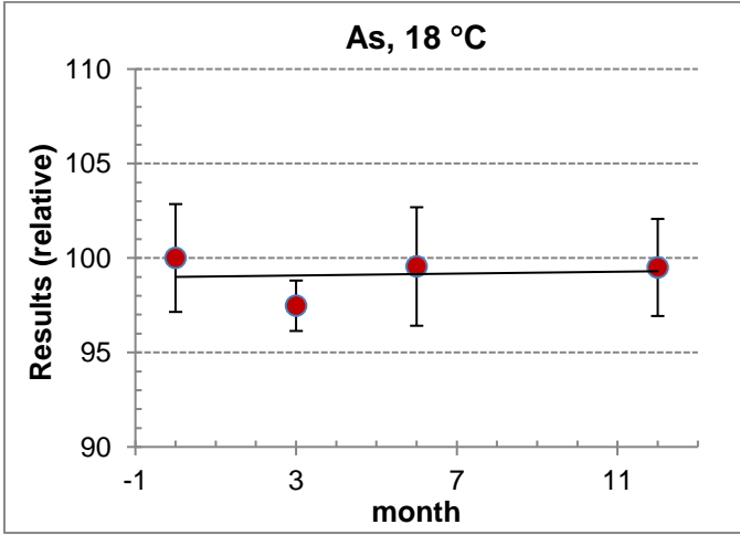
Figure A4.1. LTS plot for As at 18 °C by UME
