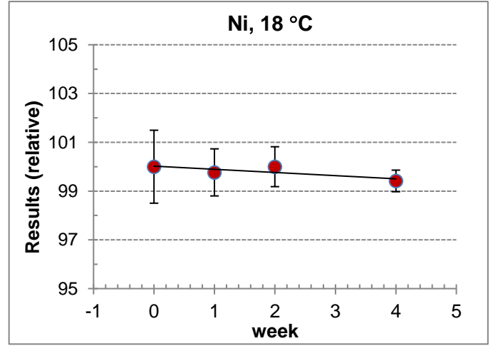
Figure A3.10. STS plot for Ni at 18 °C by IJS
