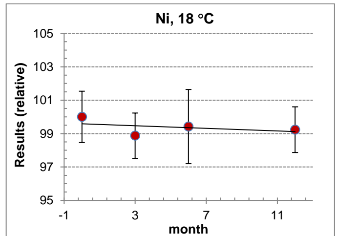
Figure A4.5. LTS plot for Ni at 18 °C by UME
