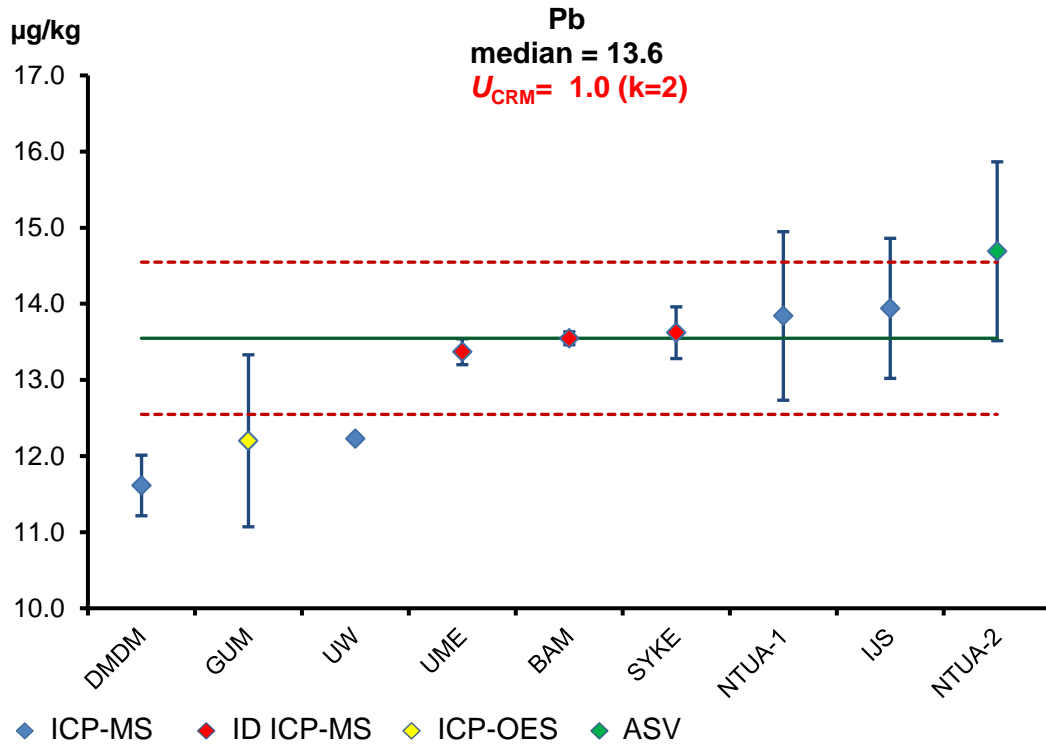
Figure A6.4. Characterization Study Plot for Pb
