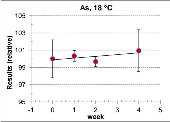
Figure A3.1. STS plot for As at 18 °C by UME
