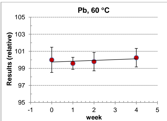
Figure A3.15. STS plot for Pb at 60 °C by UME
