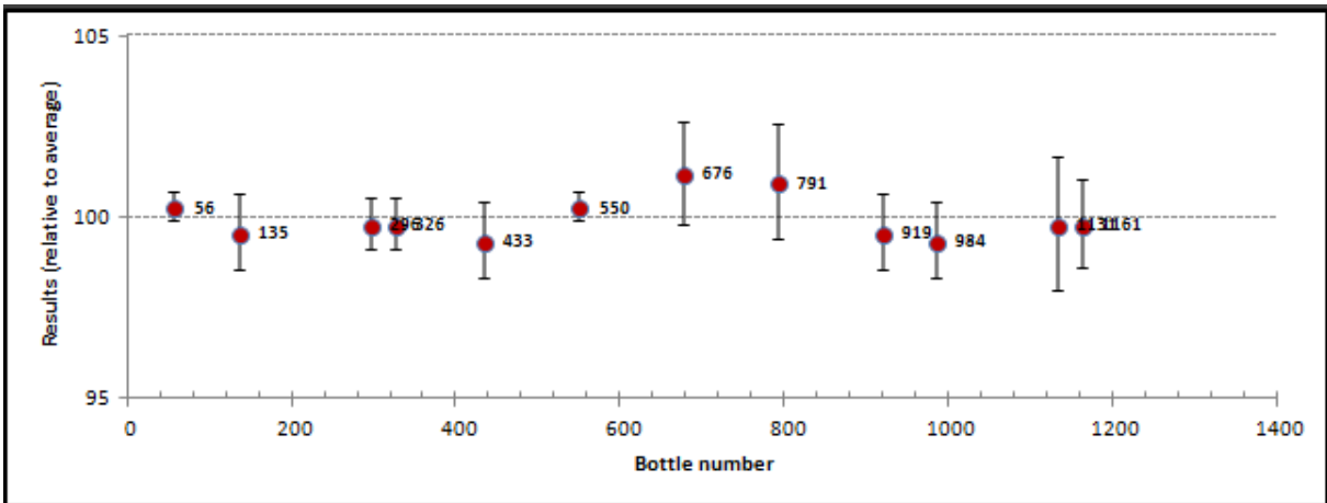
Figure A2.6. Homogeneity plot for Ni by IJS
