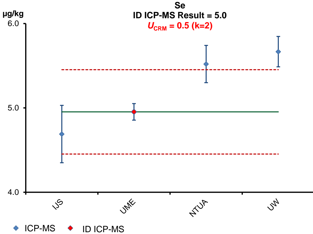
Figure A6.5. Characterization Study Plot for Se
