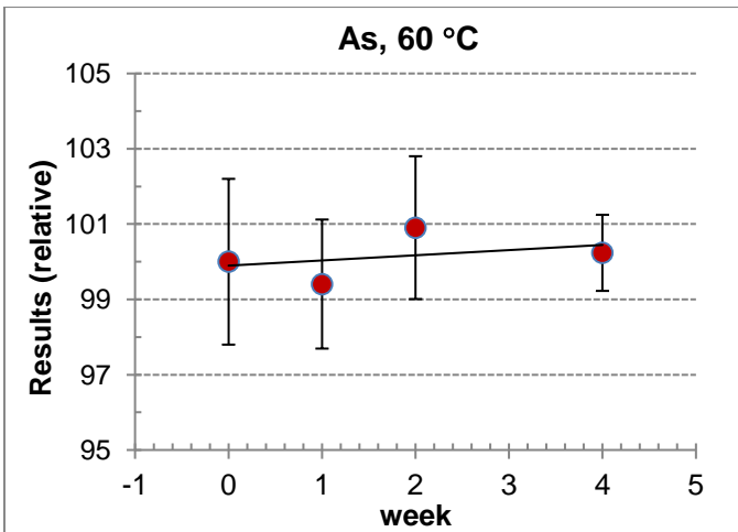
Figure A3.3. STS plot for As at 60 °C by UME
