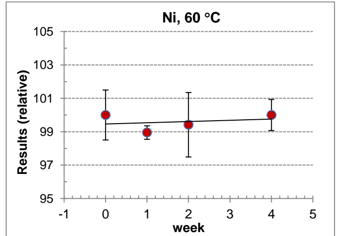
Figure A3.12. STS plot for Ni at 60 °C by IJS
