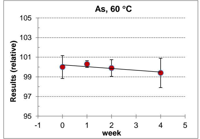
Figure A3.4. STS plot for As at 60 °C by IJS
