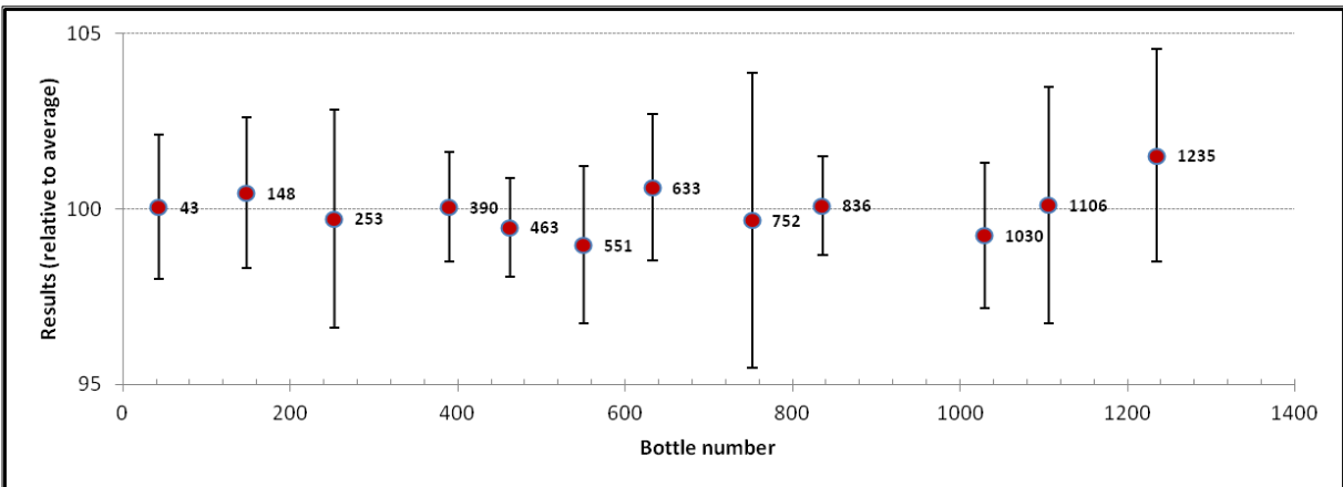
Figure A2.9. Homogeneity plot for Se by UME
