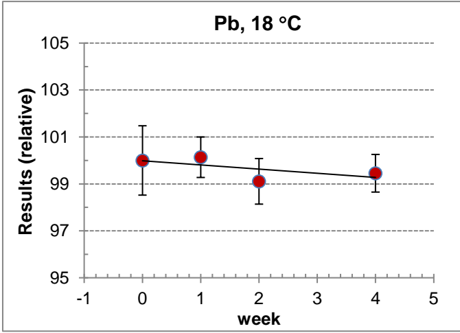
Figure A3.13. STS plot for Pb at 18 °C by UME
