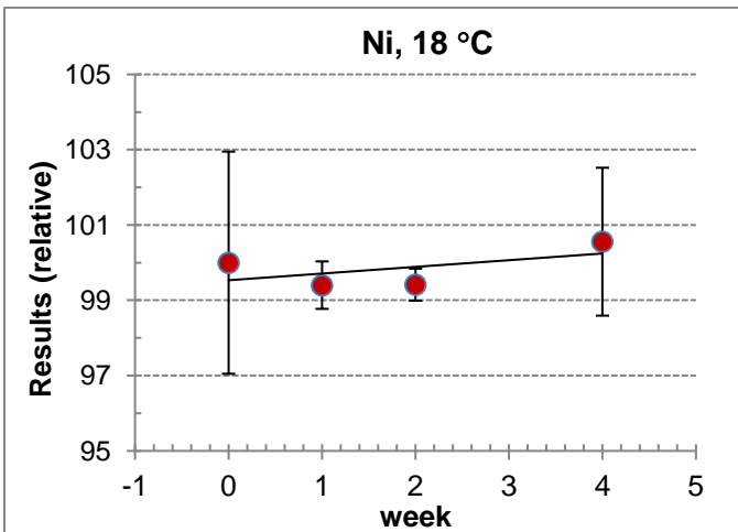
Figure A3.9. STS plot for Ni at 18 °C by UME
