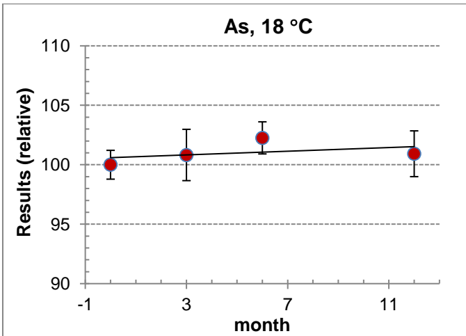
Figure A4.2. LTS plot for As at 18 °C by IJS
