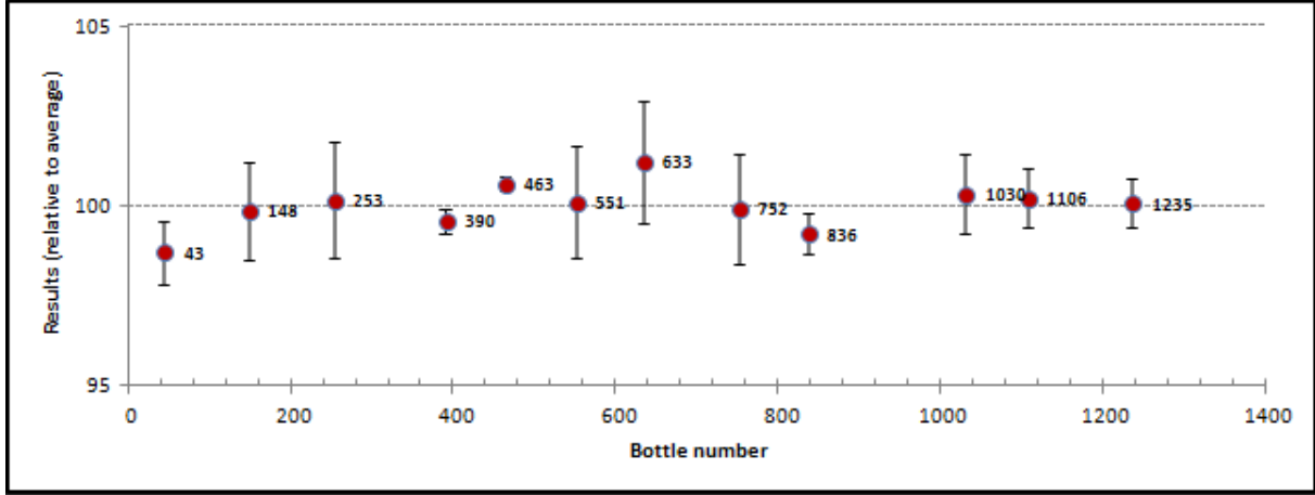
Figure A2.1. Homogeneity plot for As by UME
