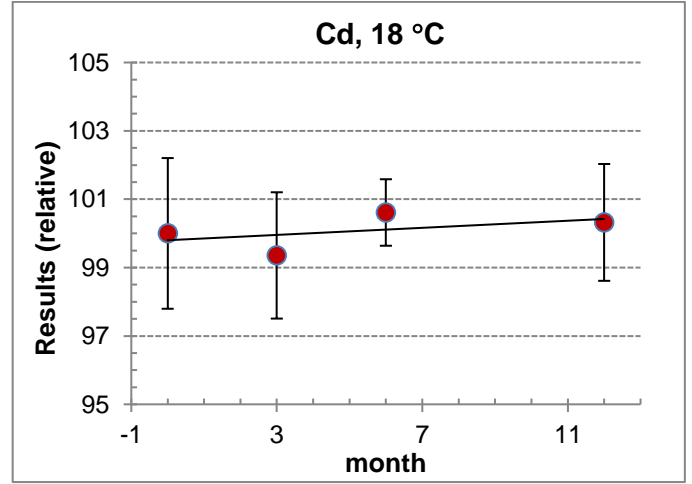
Figure A4.4. LTS plot for Cd at 18 °C by IJS
