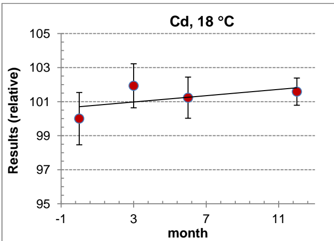
Figure A4.3. LTS plot for Cd at 18 °C by UME
