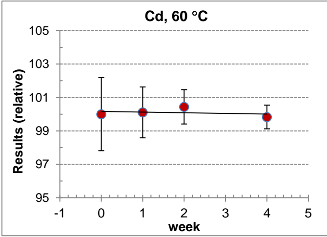
Figure A3.7. STS plot for Cd at 60 °C by UME
