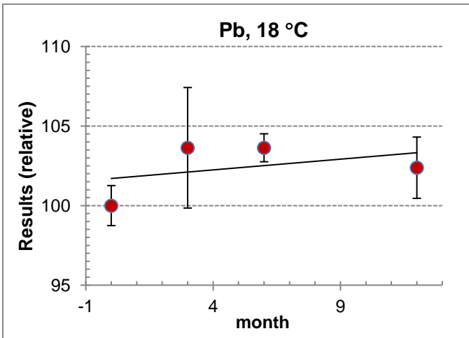
Figure A4.8. LTS plot for Pb at 18 °C by IJS
