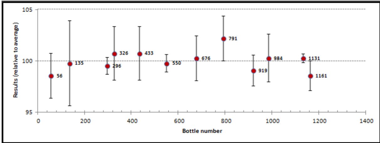
Figure A2.8. Homogeneity plot for Pb by IJS
