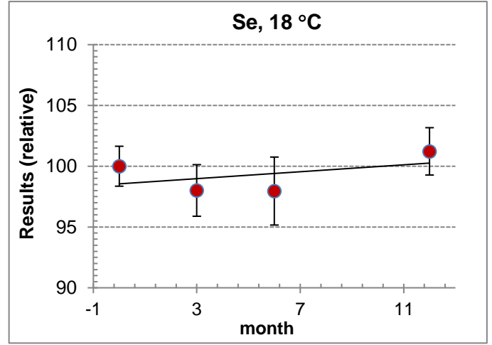
Figure A4.9. LTS plot for Se at 18 °C by UME
