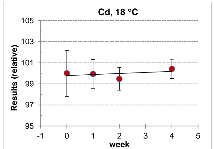
Figure A3.5. STS plot for Cd at 18 °C by UME
