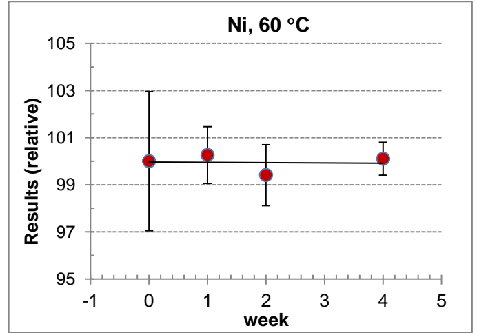
Figure A3.11. STS plot for Ni at 60 °C by UME
