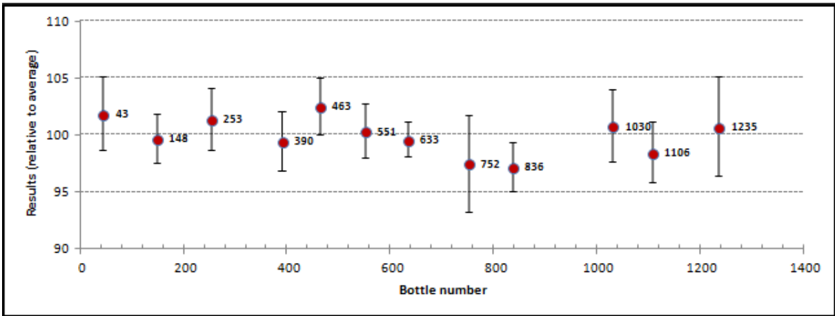
Figure A2.5. Homogeneity plot for Ni by UME
