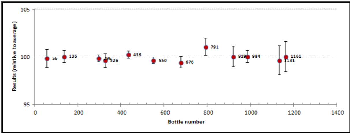
Figure A2.2. Homogeneity plot for As by IJS
