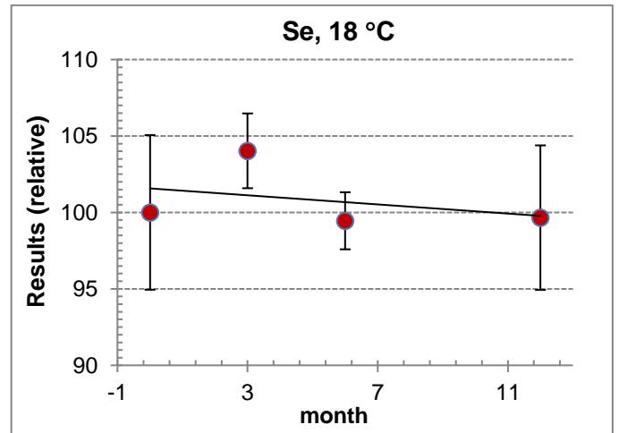
Figure A4.10. LTS plot for Se at 18 °C by IJS
