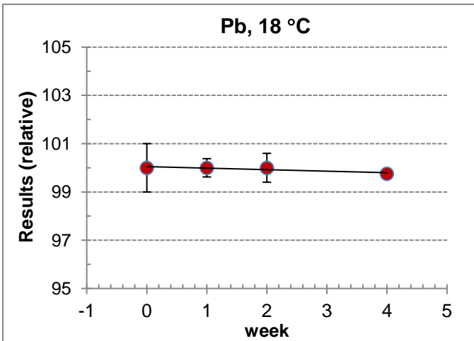
Figure A3.14. STS plot for Pb at 18 °C by IJS
