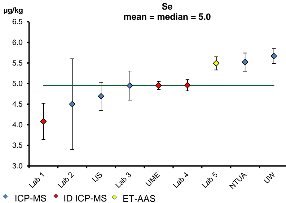
Figure A7.1. Supplementary Comparison Study Plot for Se
