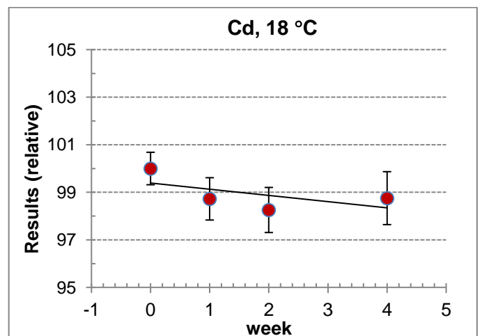
Figure A3.6. STS plot for Cd at 18 °C by IJS
