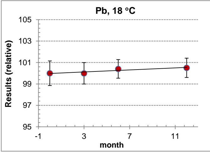
Figure A4.7. LTS plot for Pb at 18 °C by UME
