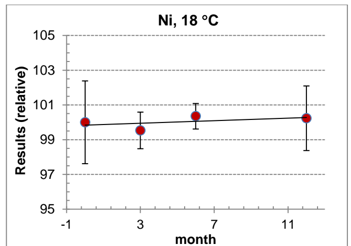
Figure A4.6. LTS plot for Ni at 18 °C by IJS
