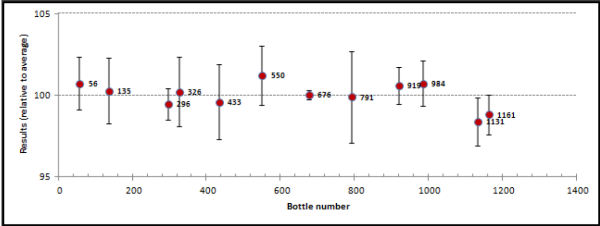
Figure A2.4. Homogeneity plot for Cd by IJS
