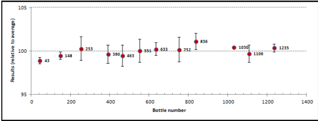
Figure A2.7. Homogeneity plot for Pb by UME
