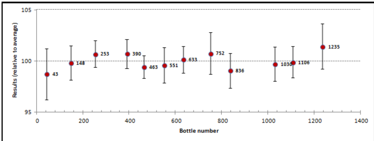
Figure A2.3. Homogeneity plot for Cd by UME
