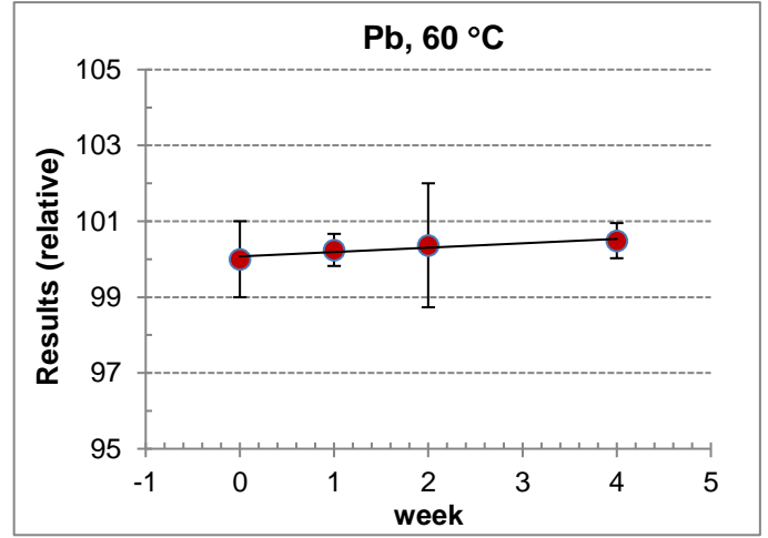
Figure A3.16. STS plot for Pb at 60 °C by IJS
