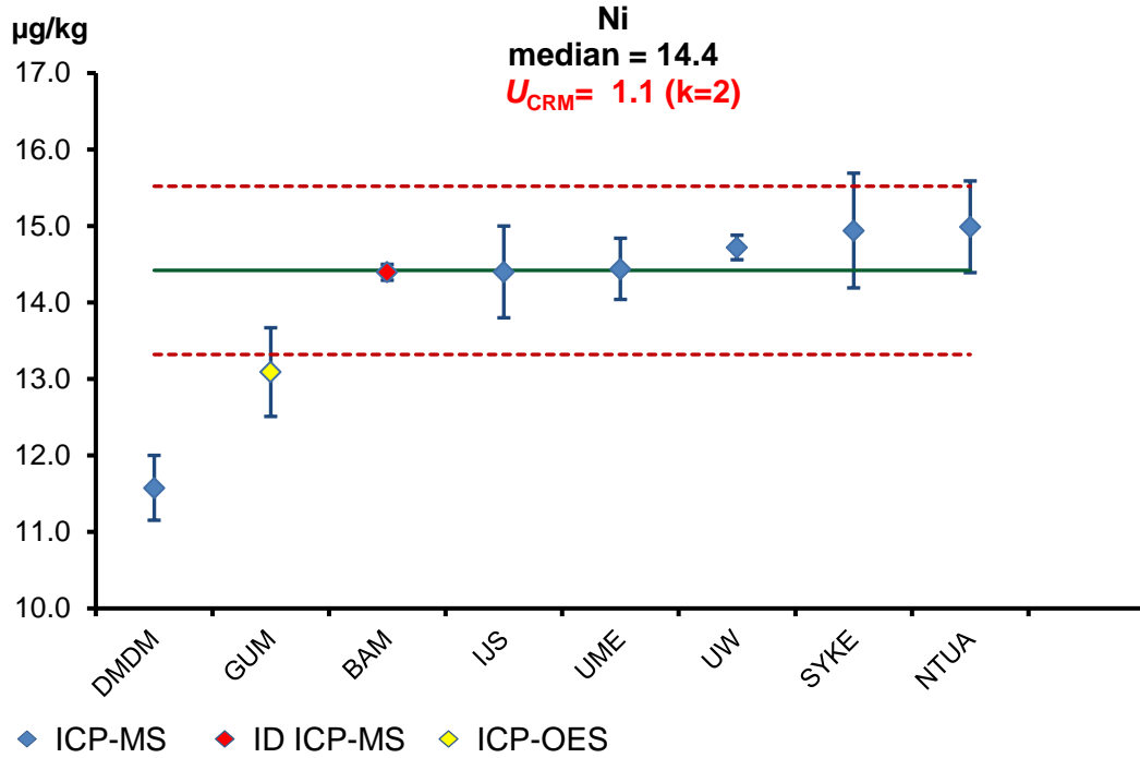
Figure A6.3. Characterization Study Plot for Ni
